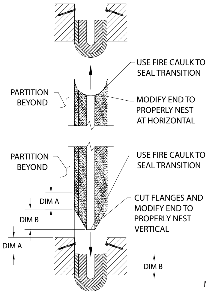
Fig 4 TRANSITION INTERSECTION DETAIL
